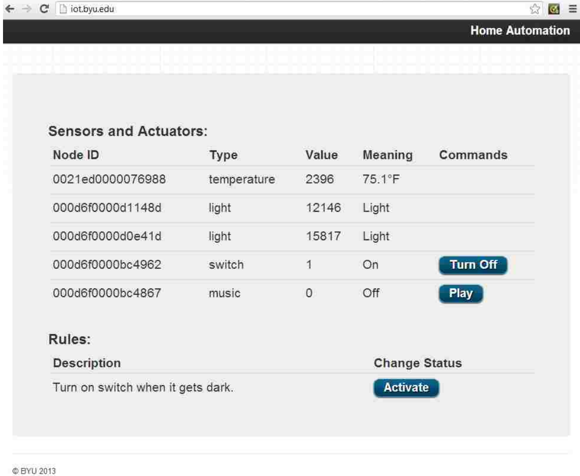
Figure 4.11: Web Browser User Interface
